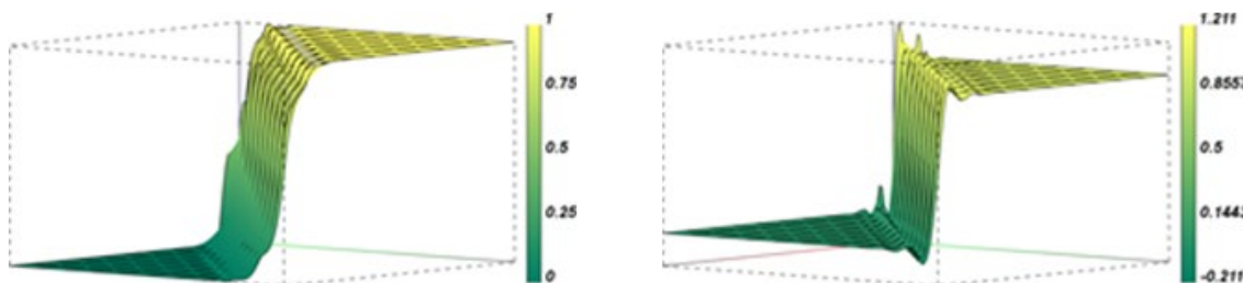
Figure 5: HO solution of the “glancing void” problem without and with the positivity-preserving S_N transport solver.
